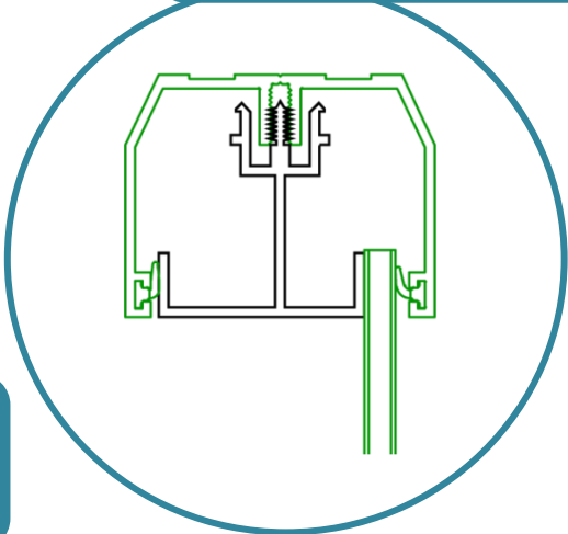
HEAD TRACK WITH GASKET SHOWN WITH OUR SINGLE WALL SYSTEM
