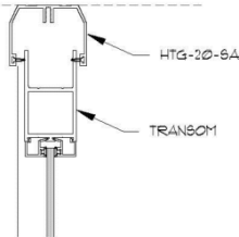
9 TRANSOM @ HEAD TRACK SCALE: 3' = 1'-0"
