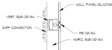
5 CONN. @ HORIZ./VERT. MEMBERS SCALE: 3' = 1'-0"
