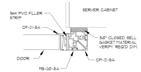
8 TYPICAL CORNER @ DOOR SCALE: 3' = 1'-0"
