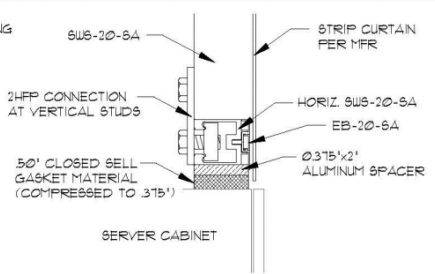
4 HDR AT CABINET/ACCESS DOOR SCALE: 3' = 1'-0"
