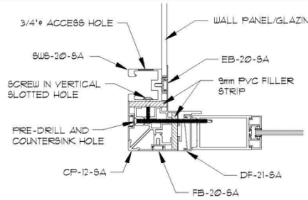
3 TYPICAL CORNER @ TRANSOM SCALE: 3' = 1'-0"
