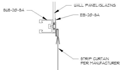
6 TOP OF ACCESS OPENING SCALE: 3' = 1'-0"
