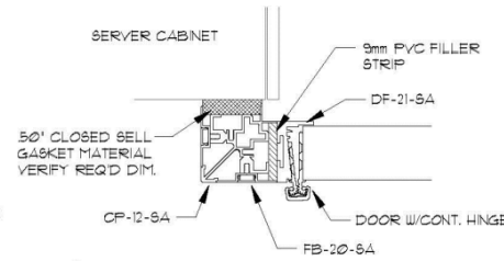
7 TYPICAL CORNER @ HINGE SCALE: 3' = 1'-0"
