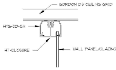
1 DEFLECTION AT GLAZING CLIP SCALE: 3' = 1'-0"
