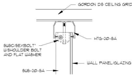
2 SUSPENDED STUD CONNECTION SCALE: 3' = 1'-0"
